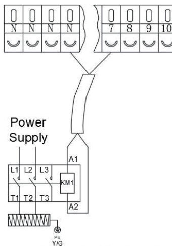
Electric Heater for Water Tank
