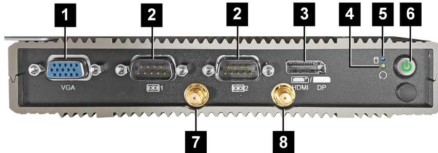
Fig. 2-1: Front view of embedded PC
